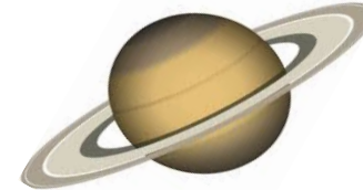
Saturn
